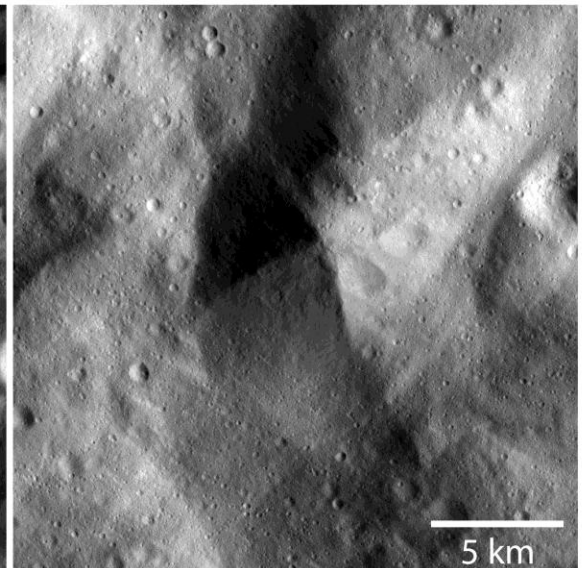
Low-Altitude Mapping Orbit (LAMO)
