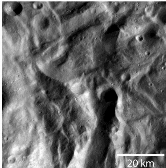
High-Altitude Mapping Orbit (HAMO)
